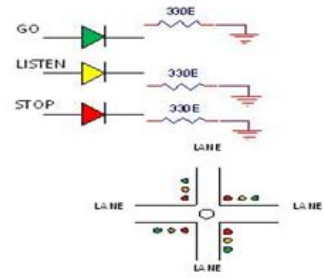
Traffic Light Controller
